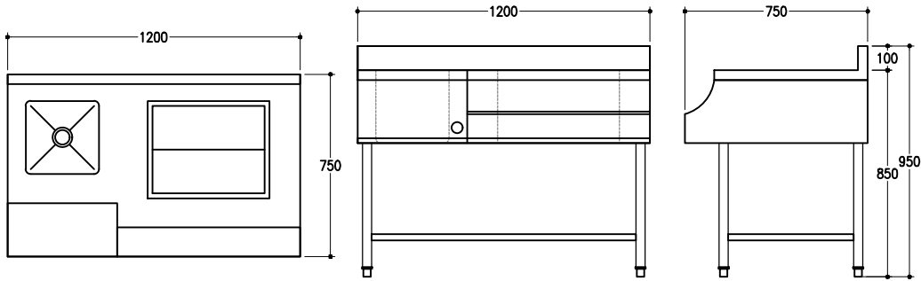
TOP VIEW
